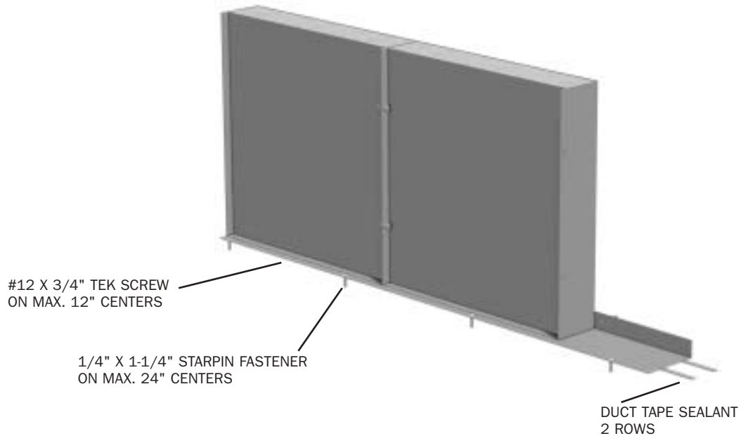
WALL PANEL TO FLOOR CONNECTION
