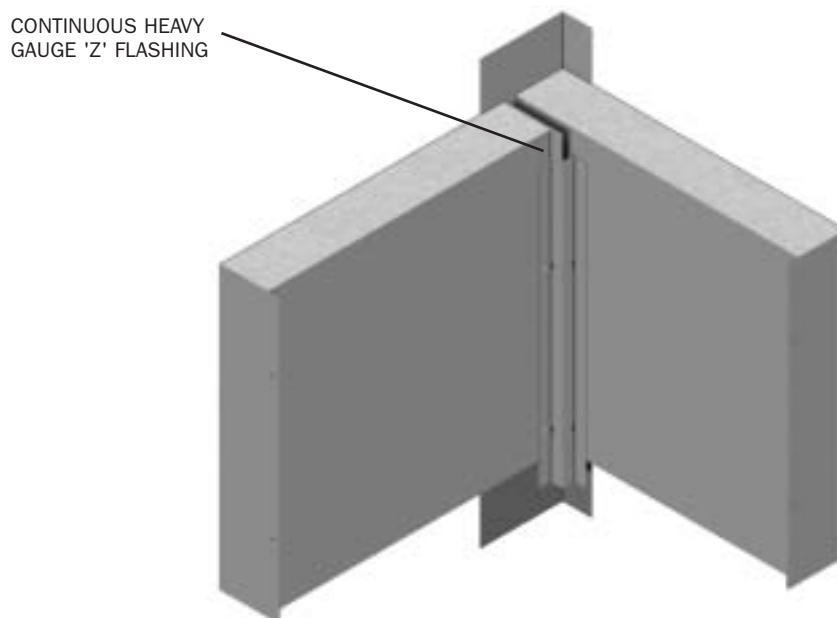
TWO PIECE CORNER
